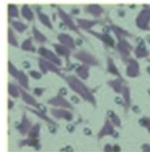
Processed
