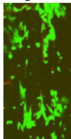
Processed
