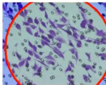
Processed Image
