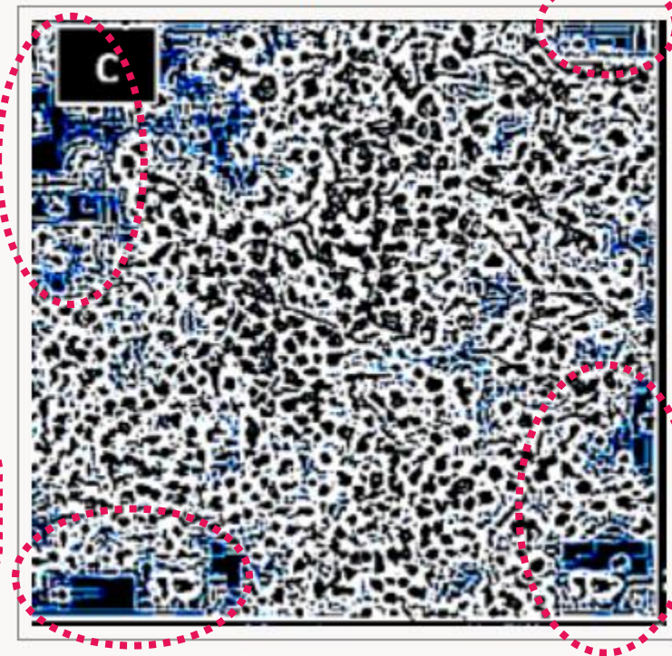
noise1_3
