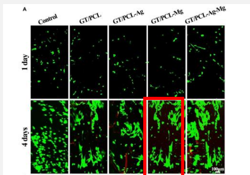
Original Image
