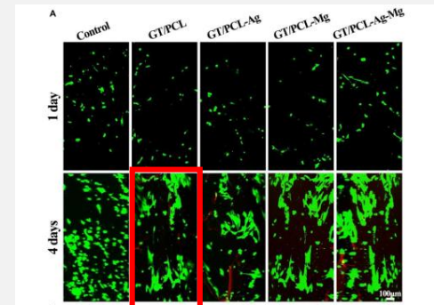
Original Image
