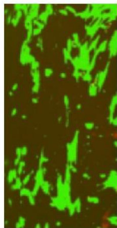
Processed Image
