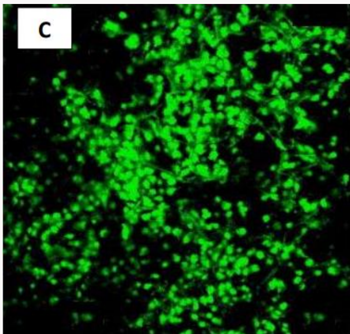
Original Image
