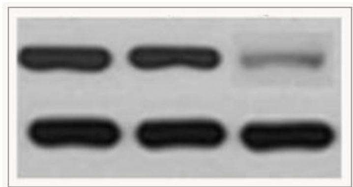
Processed Image
