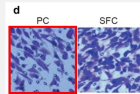
Original Image
