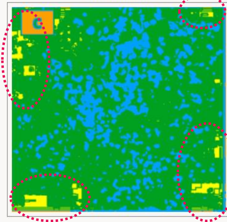
Beautification
